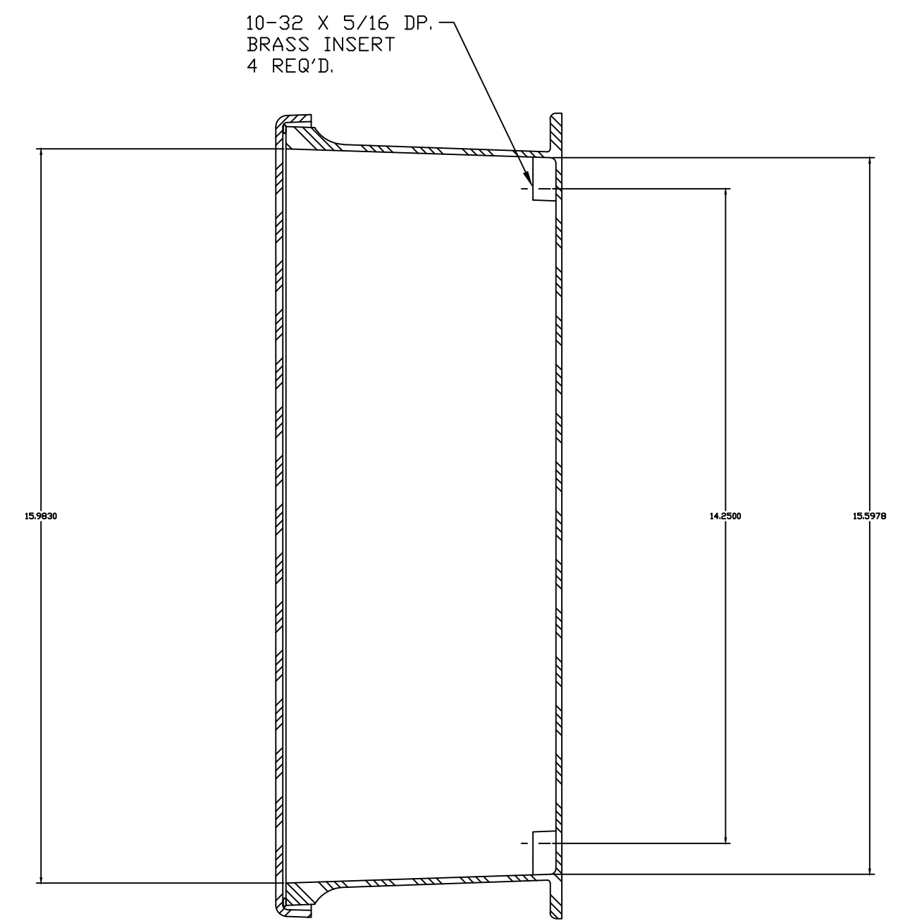
SECTION B-B
