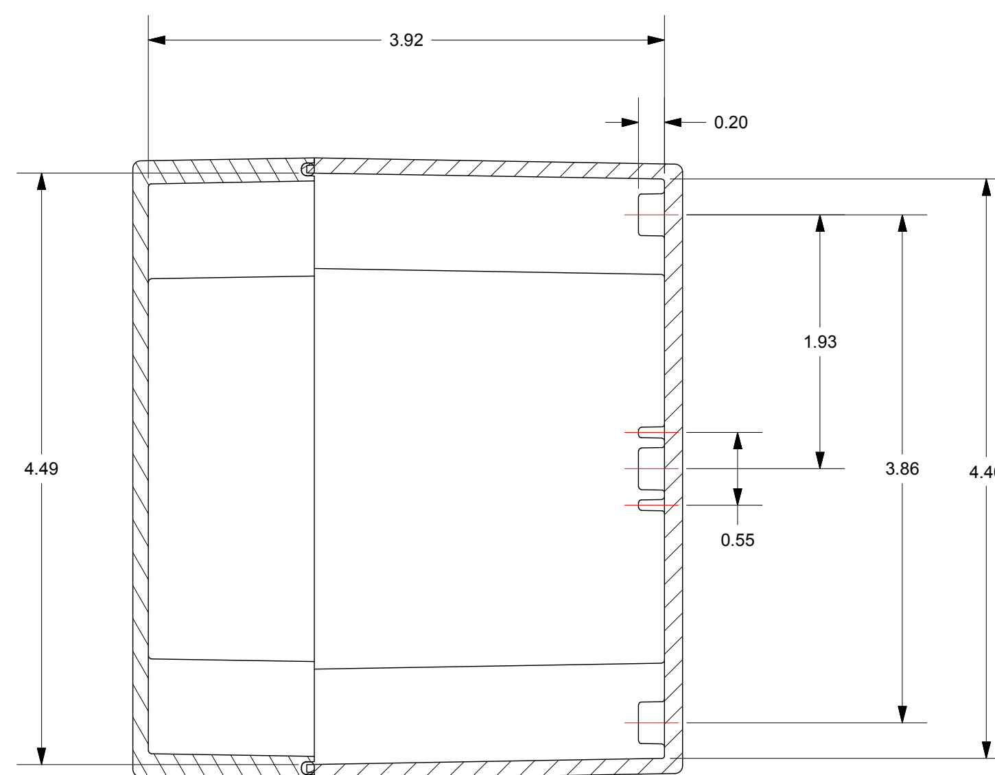
SECTION B-B
