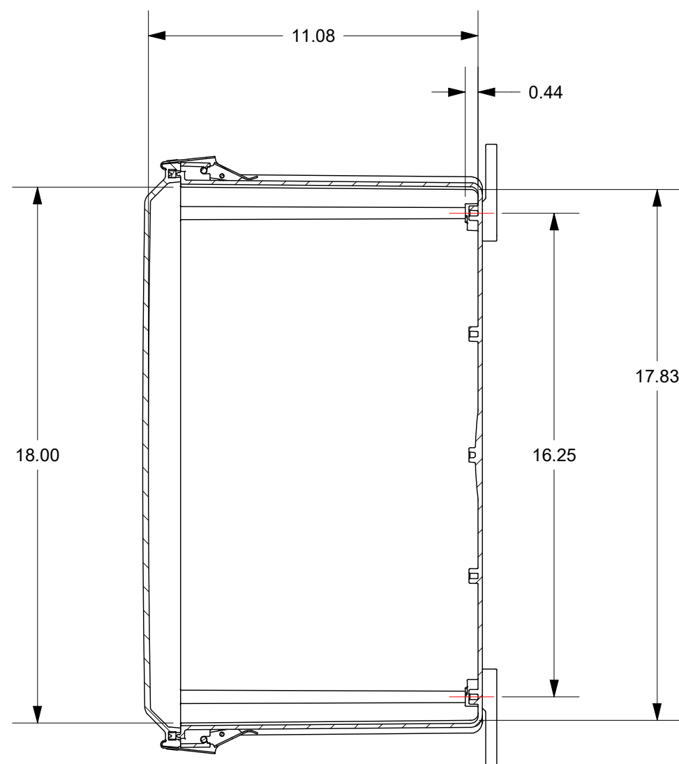
SECTION B-B
