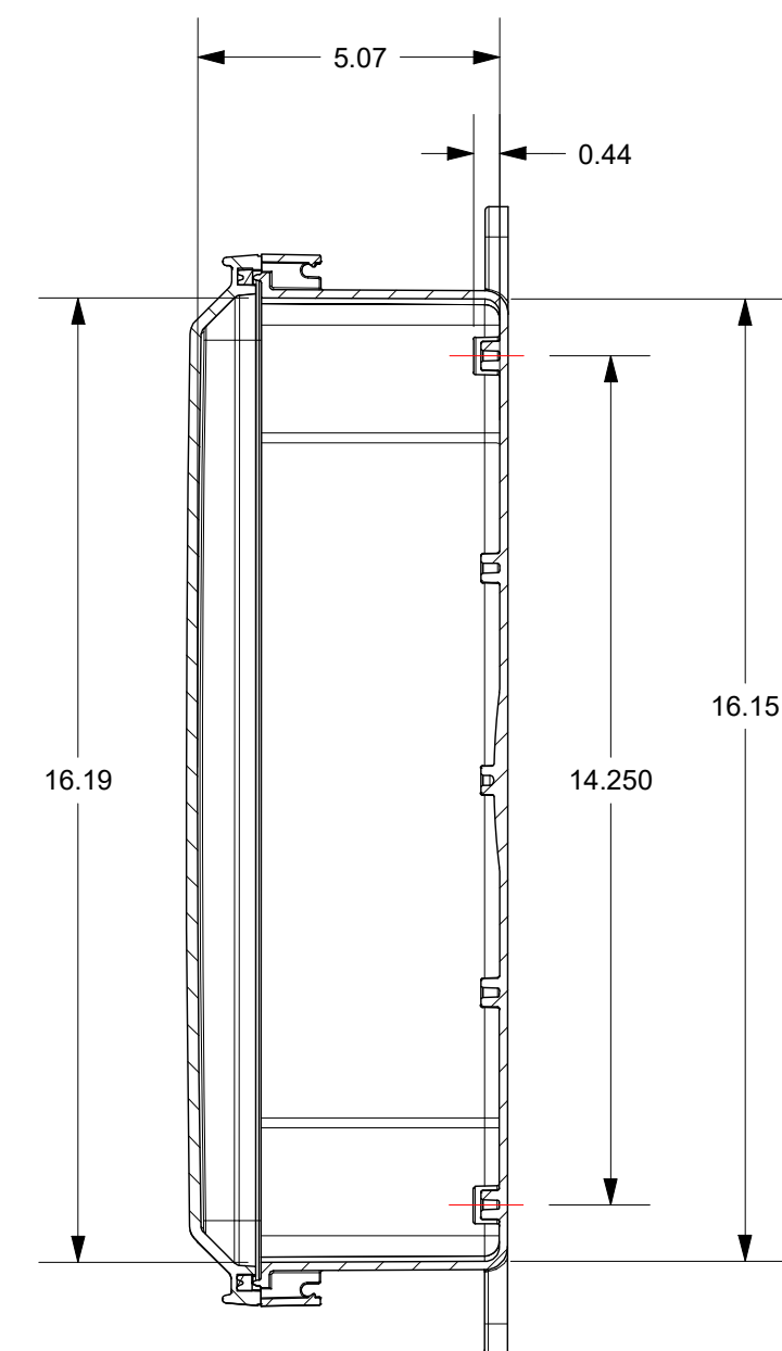
SECTION B-B
