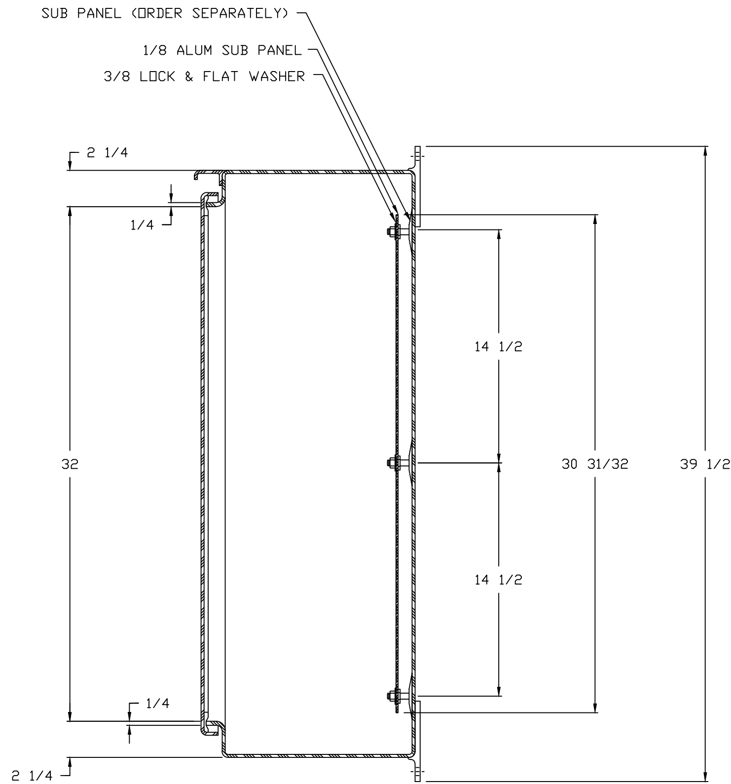
SECTION B-B
