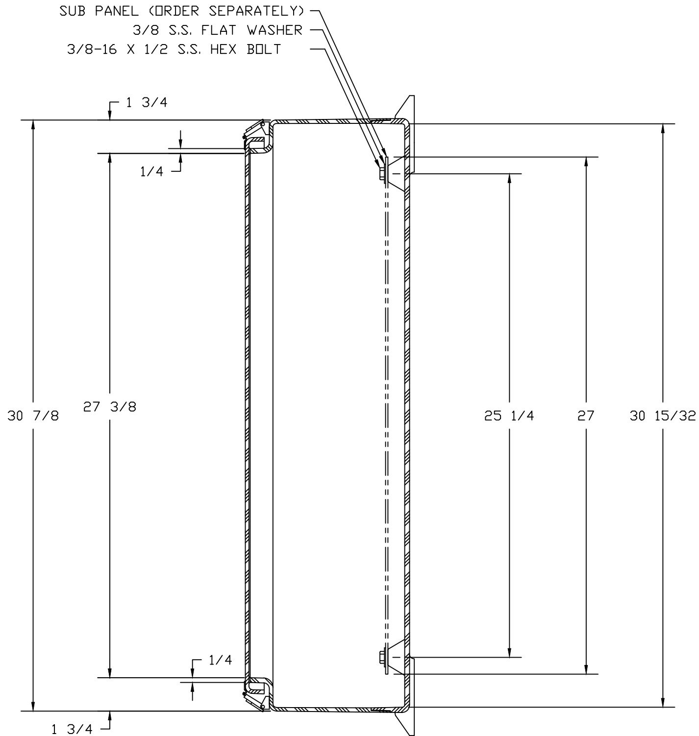
SECTION B-B
