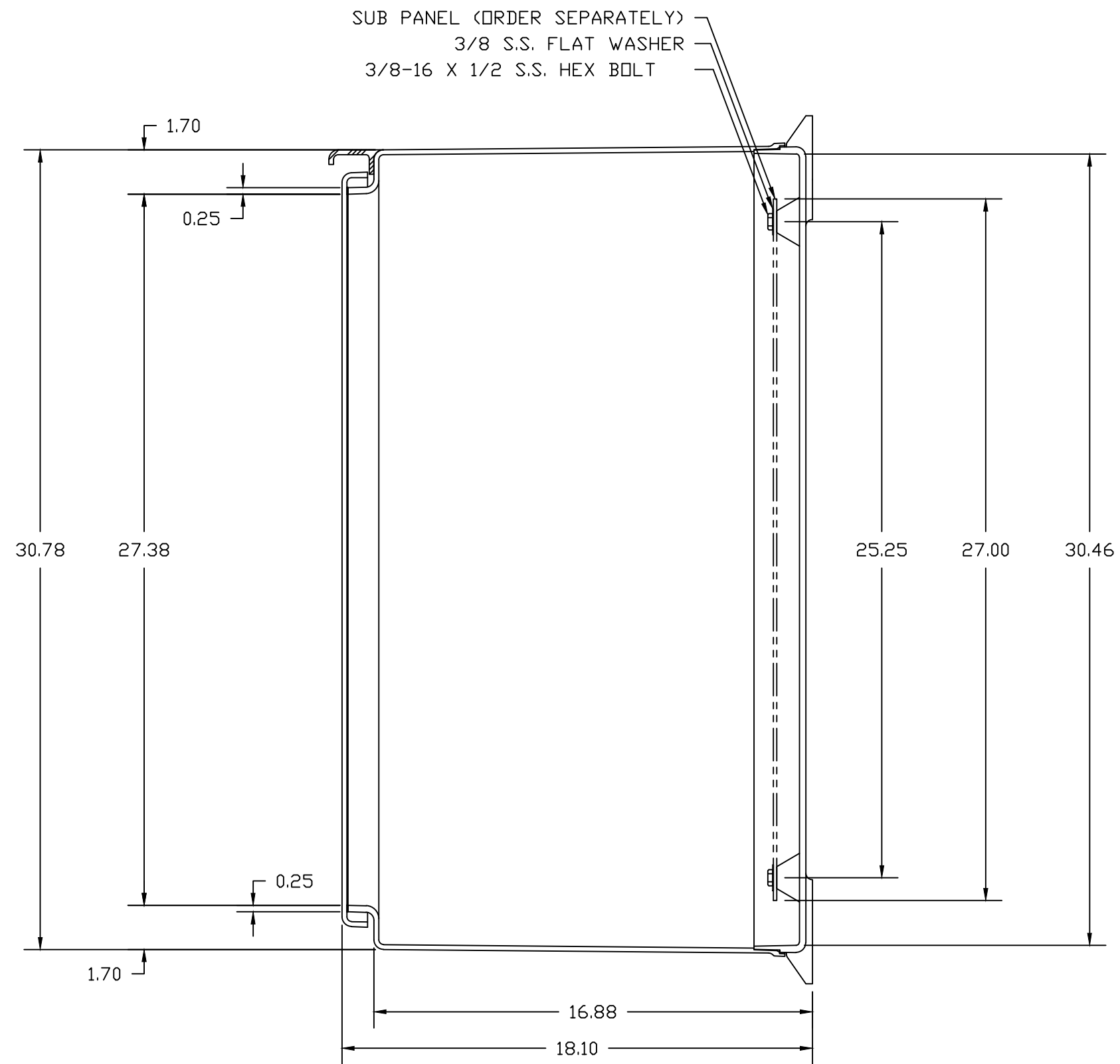
SECTION B-B
