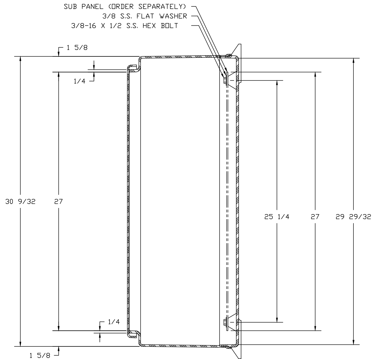
SECTION B-B
