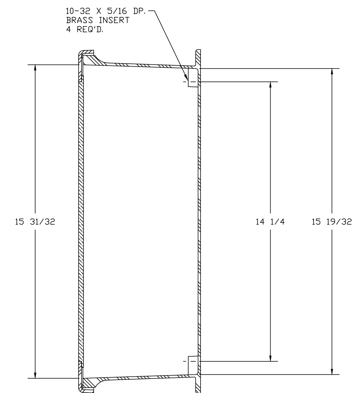
SECTION B-B
