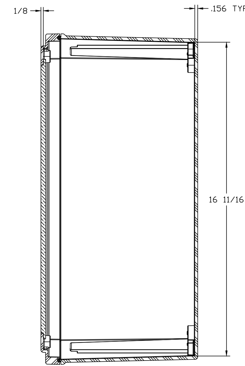
SECTION B-B
