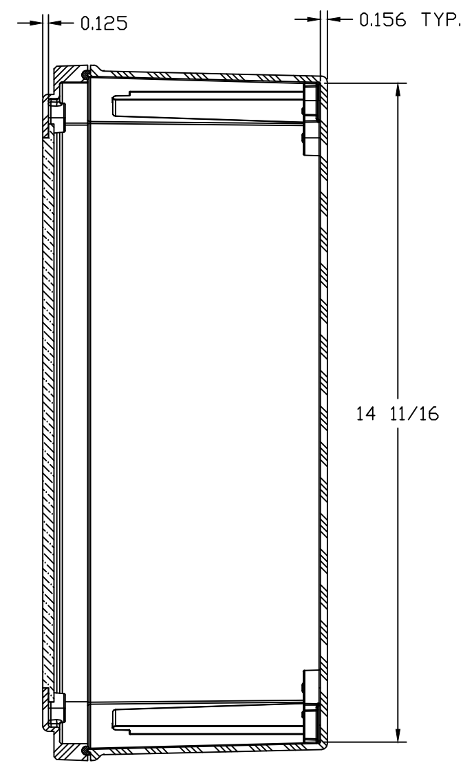
SECTION B-B
