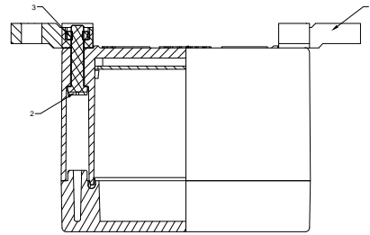
SECTION H-H SCALE 1:1
