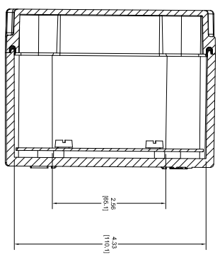
SECTION E-E SCALE 1:1
