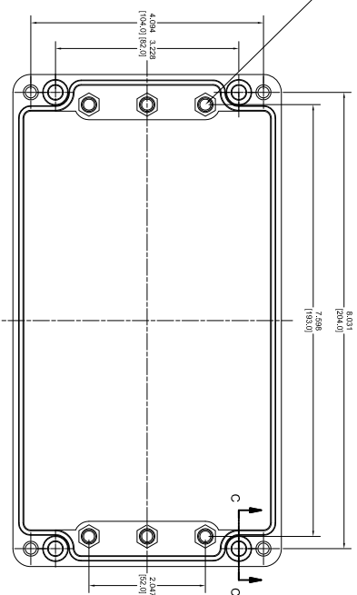
TOP VIEW WITHOUT COVER
