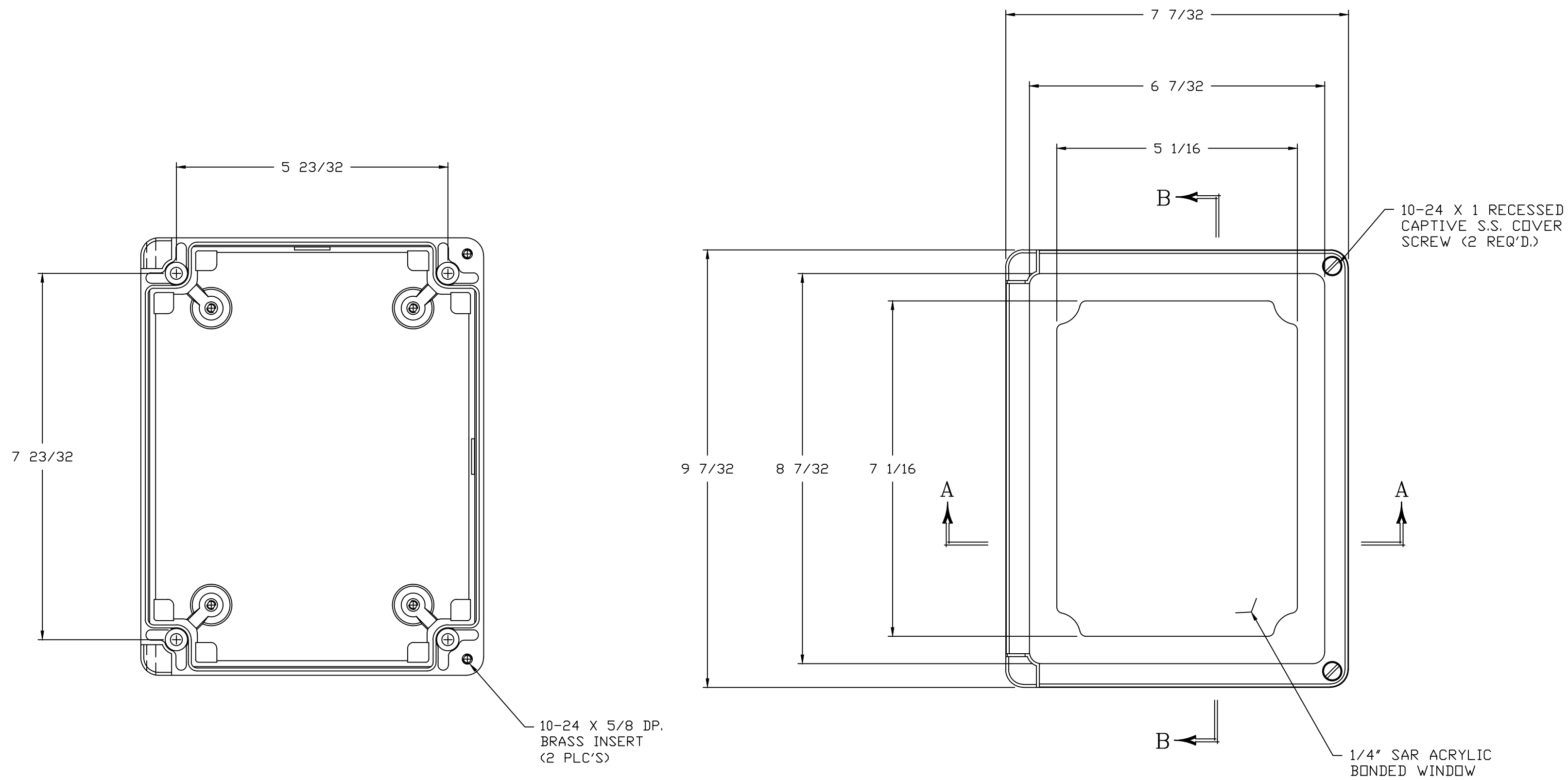
INSIDE VIEW WITHOUT COVER
