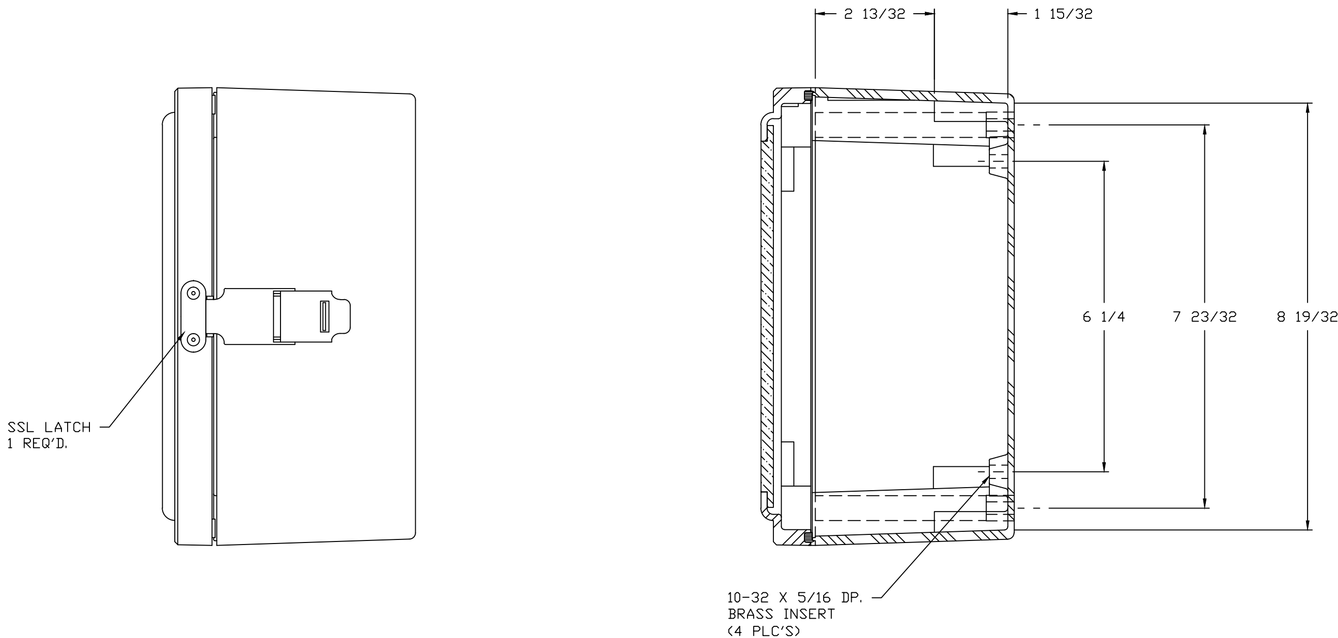
SECTION B-B
