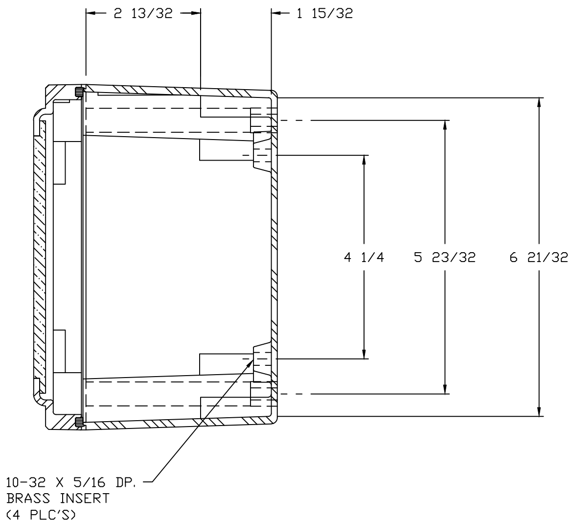
SECTION B-B
