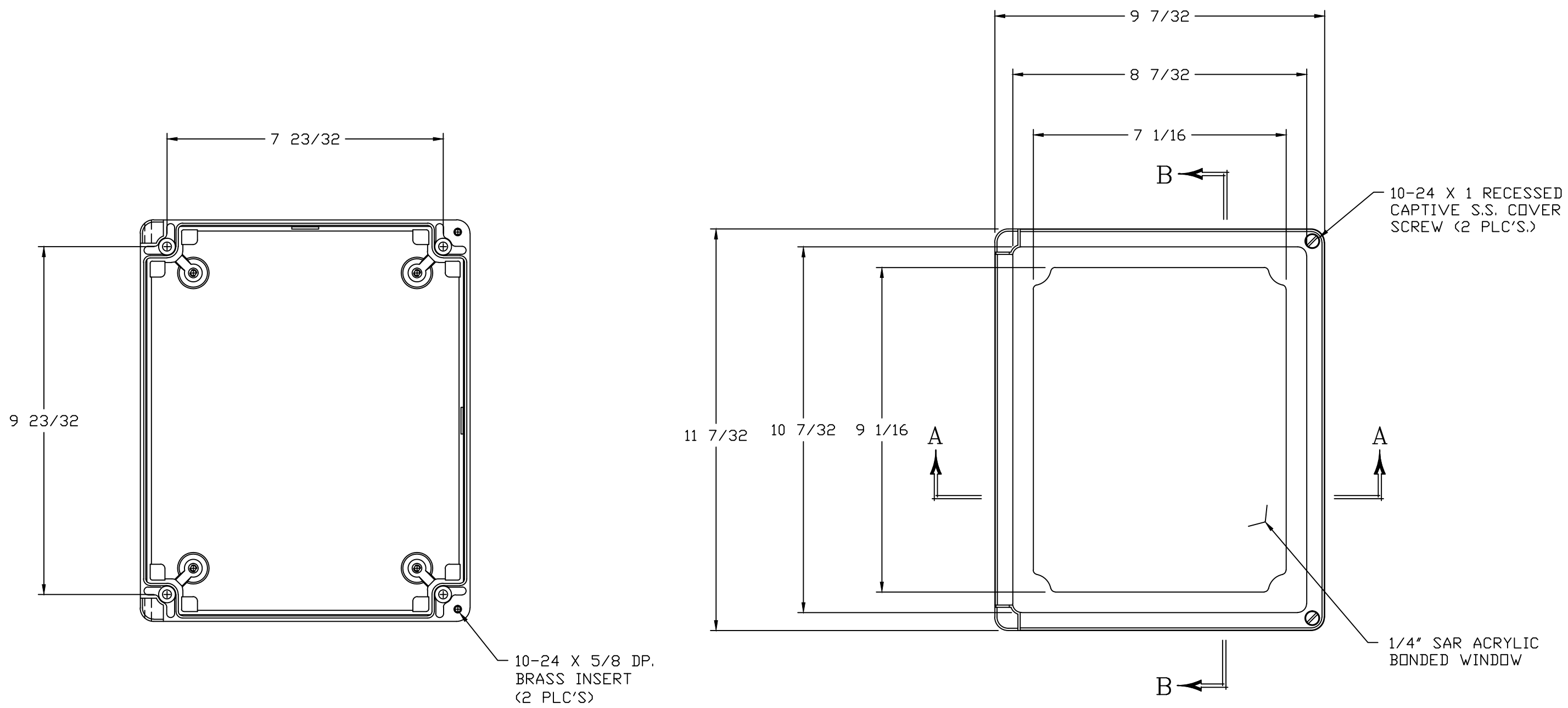
INSIDE VIEW WITHOUT COVER
