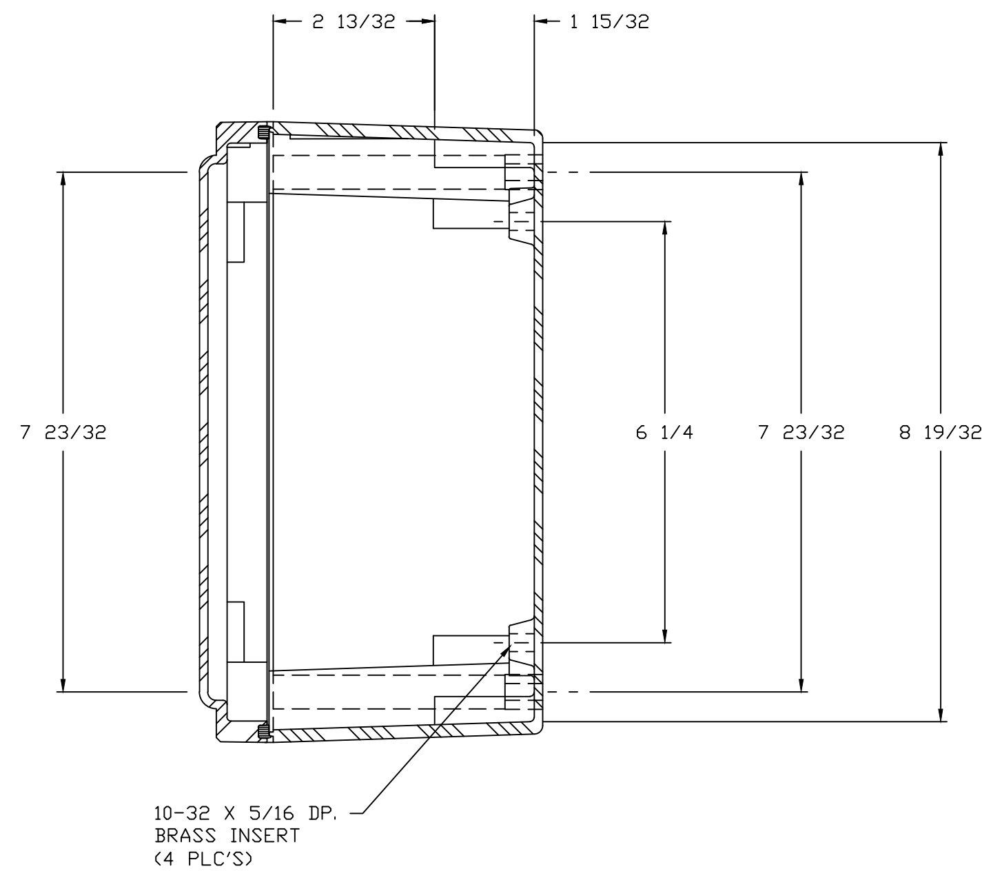
SECTION B-B
