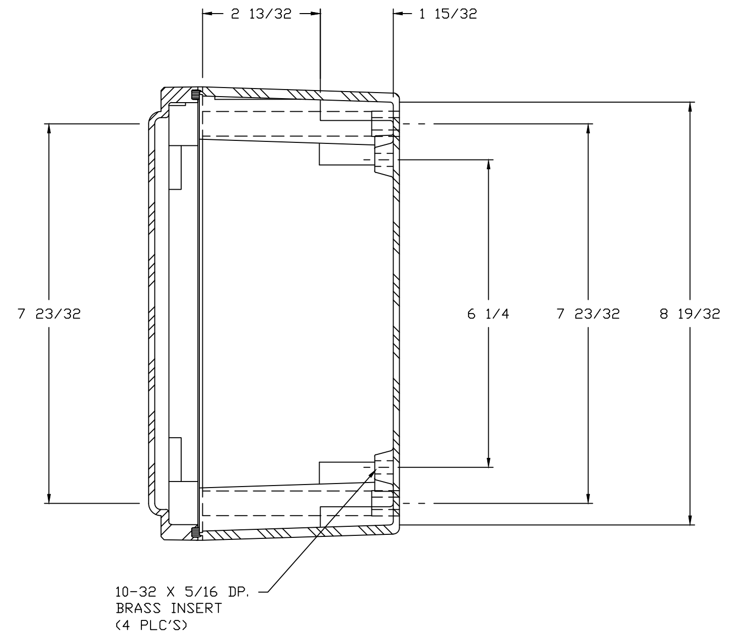
SECTION B-B
