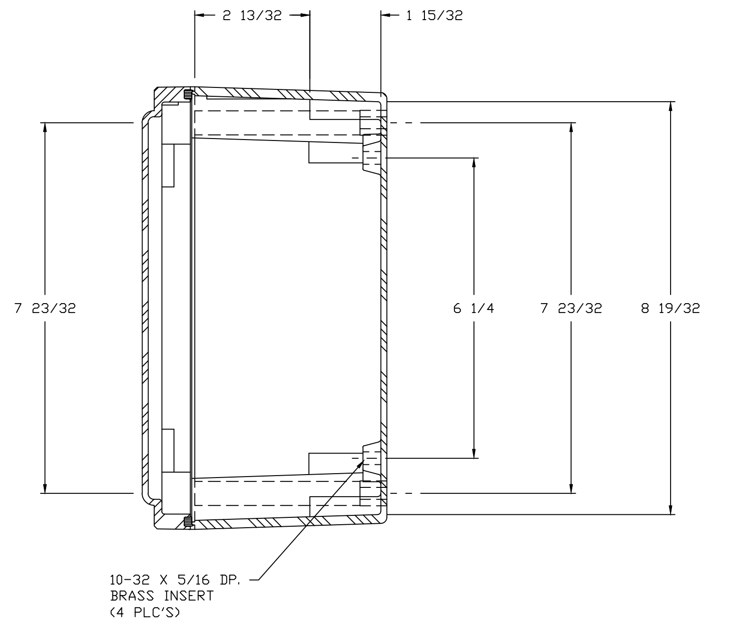
SECTION B-B
