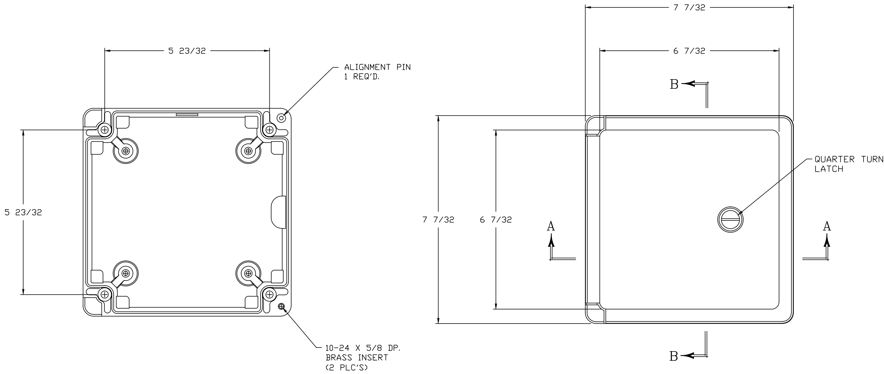
INSIDE VIEW WITHOUT COVER
