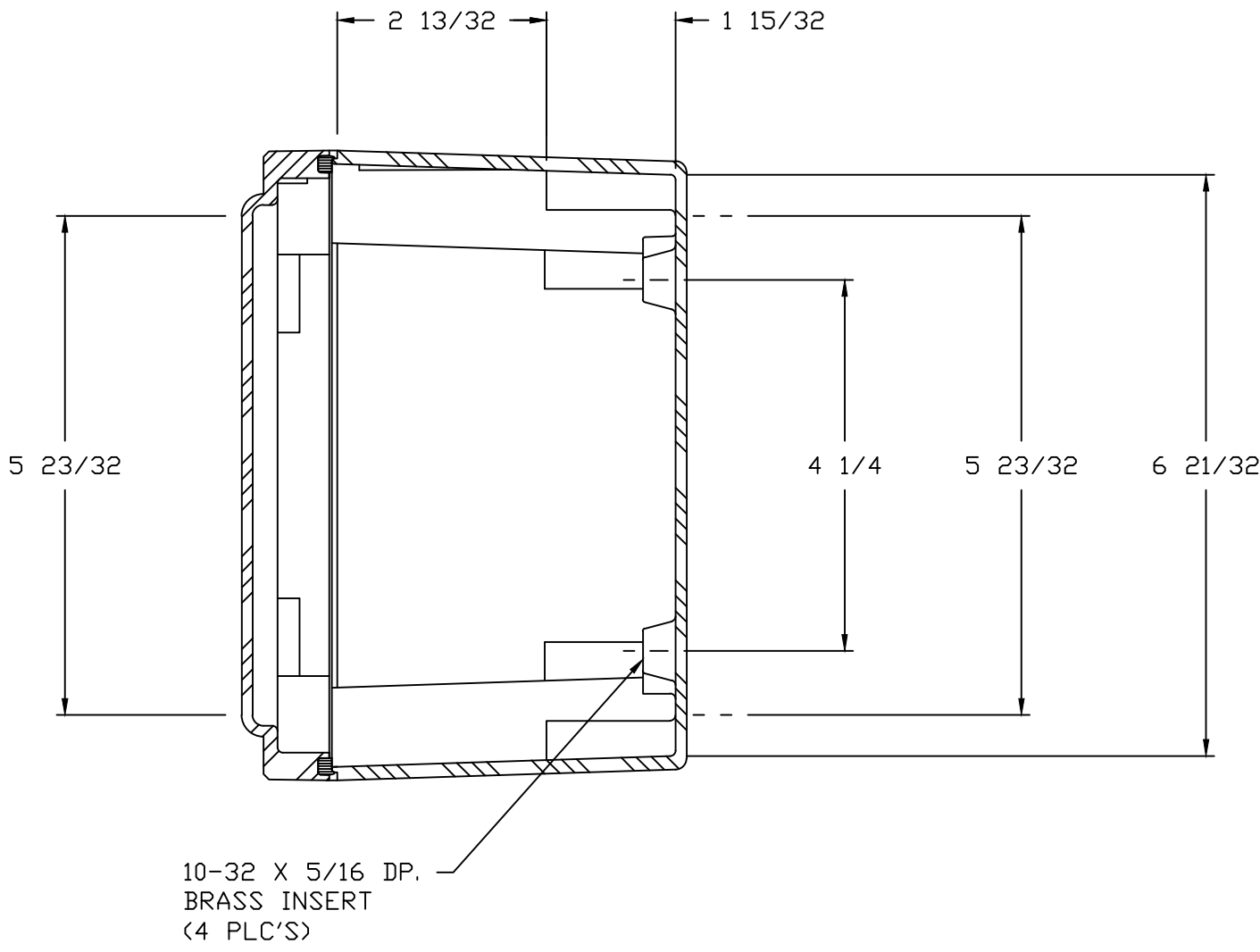
SECTION B-B
