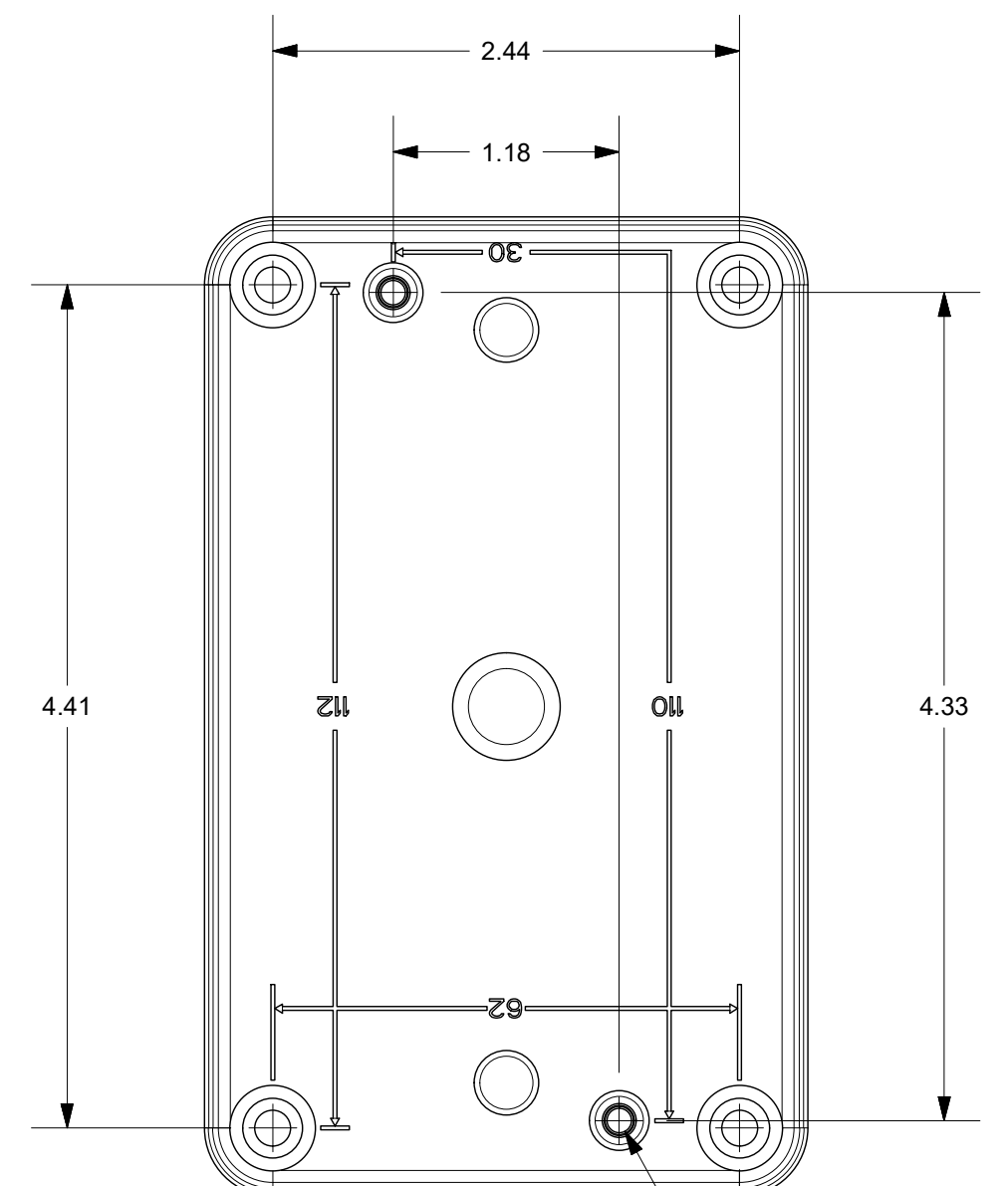
BACK VIEW
