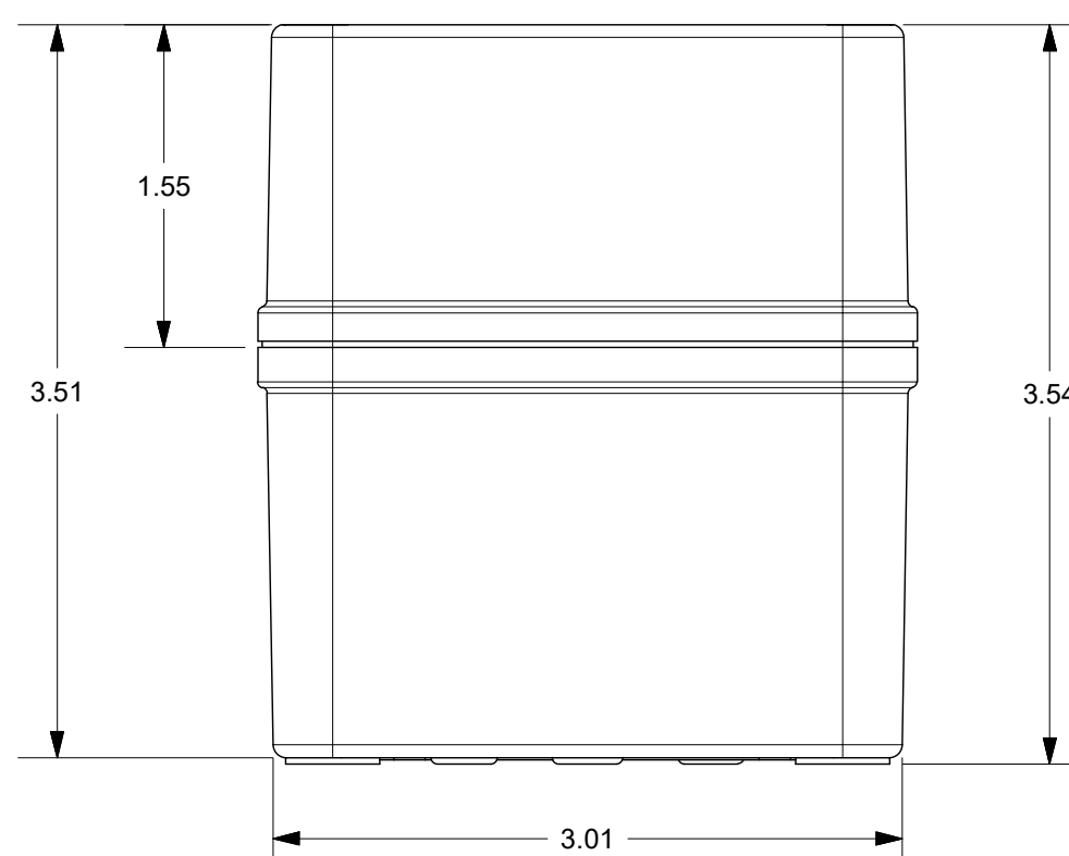
BOTTOM VIEW
