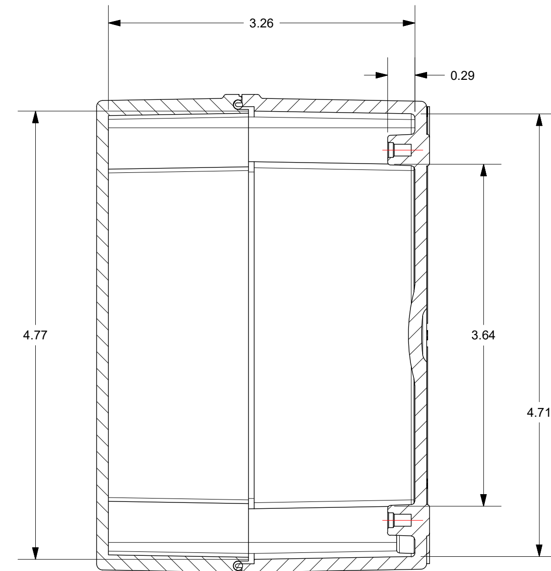
SECTION B-B
