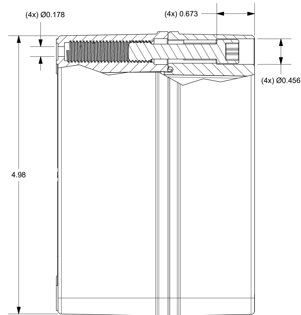
LEFT VIEW
