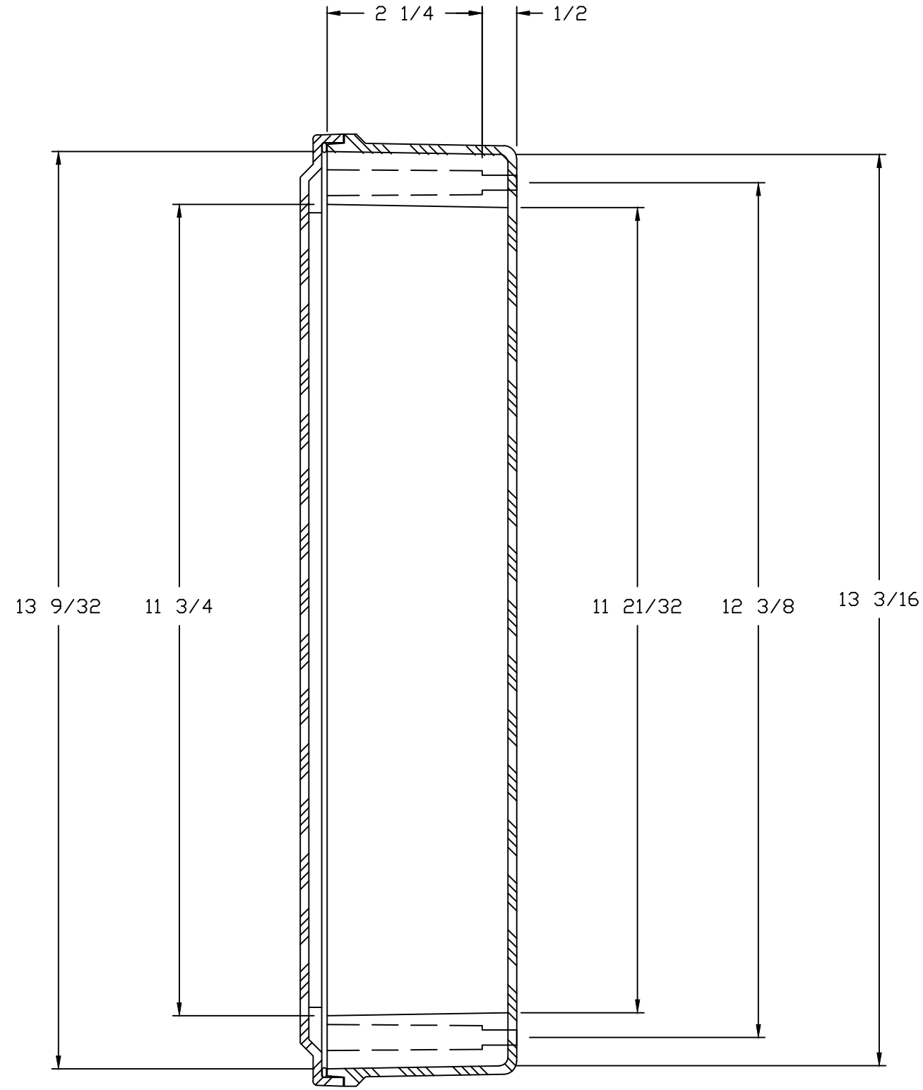
SECTION B-B
