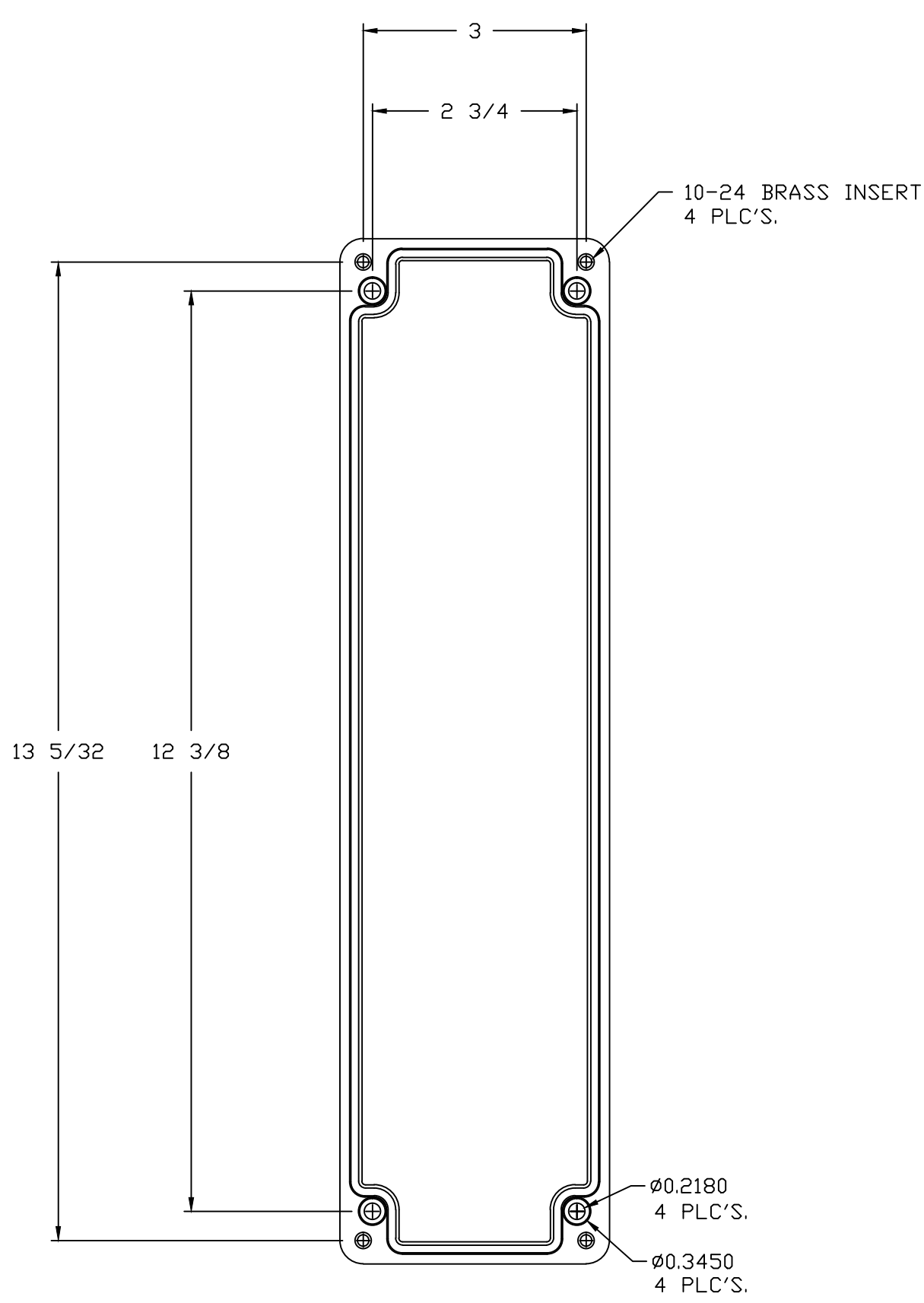
TOP VIEW WITHOUT COVER
